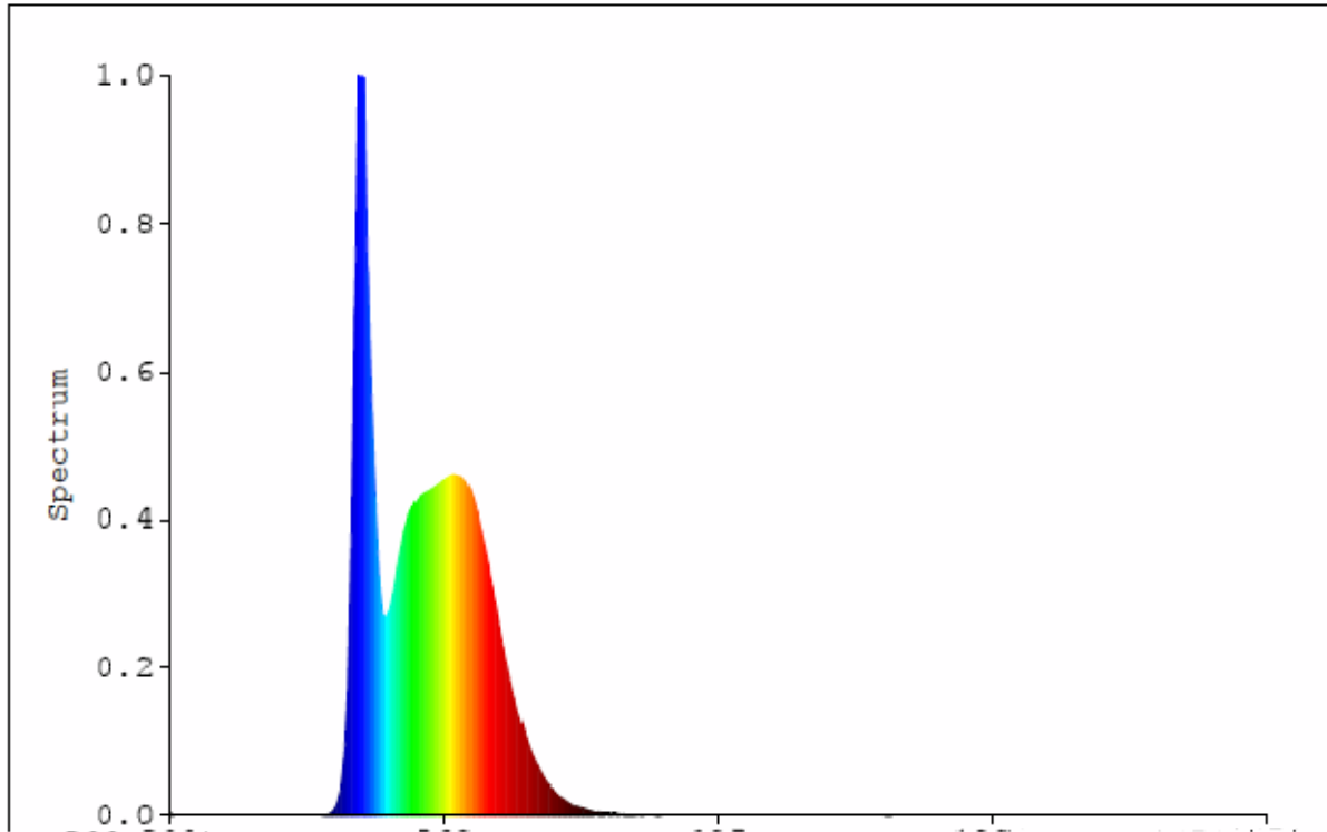
Figure of Spectral distribution
